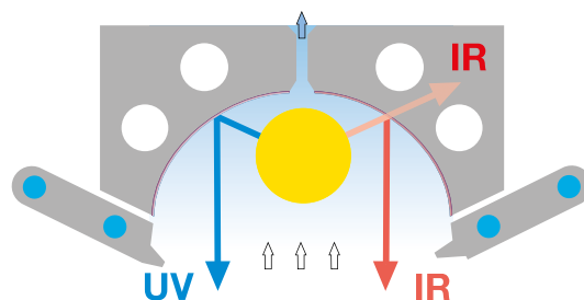
URS®-A reflector system
